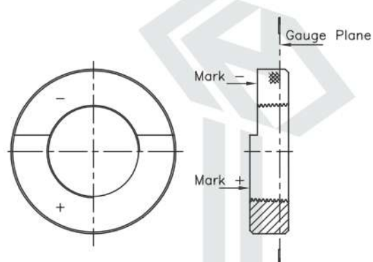
BSPT r System B Ring
