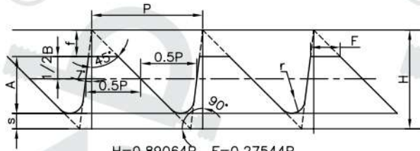
BUTTRESS 7/45° THREAD PROFILE
