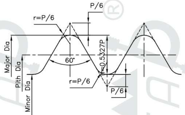
B.S. CYCLE THREAD PROFILE
