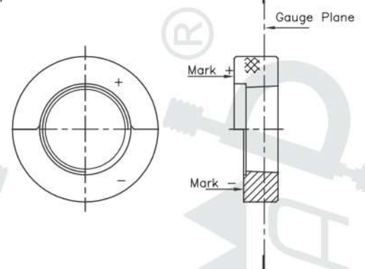
Taper Plain Ring Gauge (without threads) Gauge No.4
