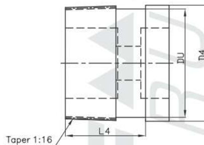
External Upset Tubing Plug Gauge
