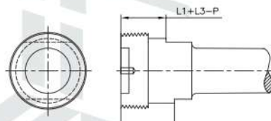
NPTF L3 Step Limit Plug (2 Step design)
