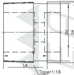
Taper Plug Gauge
