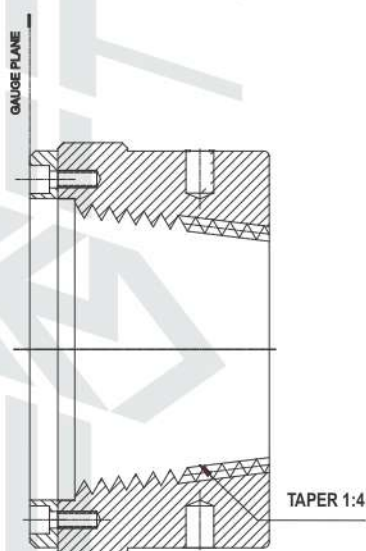
BECO THREAD RING
