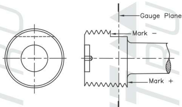
BSPT r System B Plug
