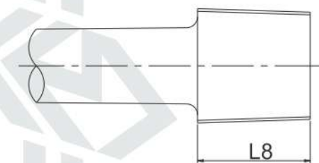
Master check Plug to check rings L1 & L8 ( M-EXT ) - IS 15894
