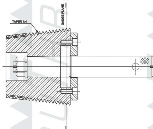
BECO THREAD PLUG ASSEMBLY
