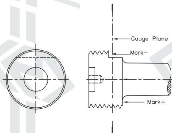
Taper Full form Thread Plug. Gauge No.1
