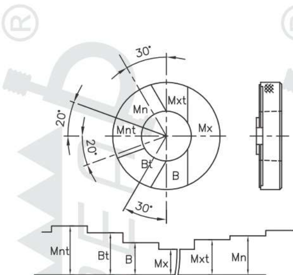
Plain Taper ring Gauge for Checking Crest Truncations of External threads (Six step design) H-28 Part II -1957
