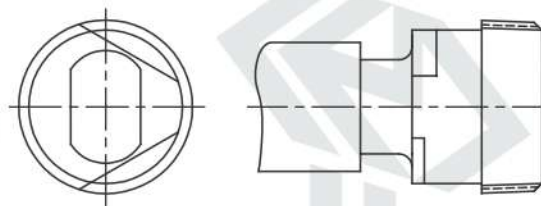
Full Form Taper Thread Plug Gauge For Checking Thread in Cylinder Neck L9
